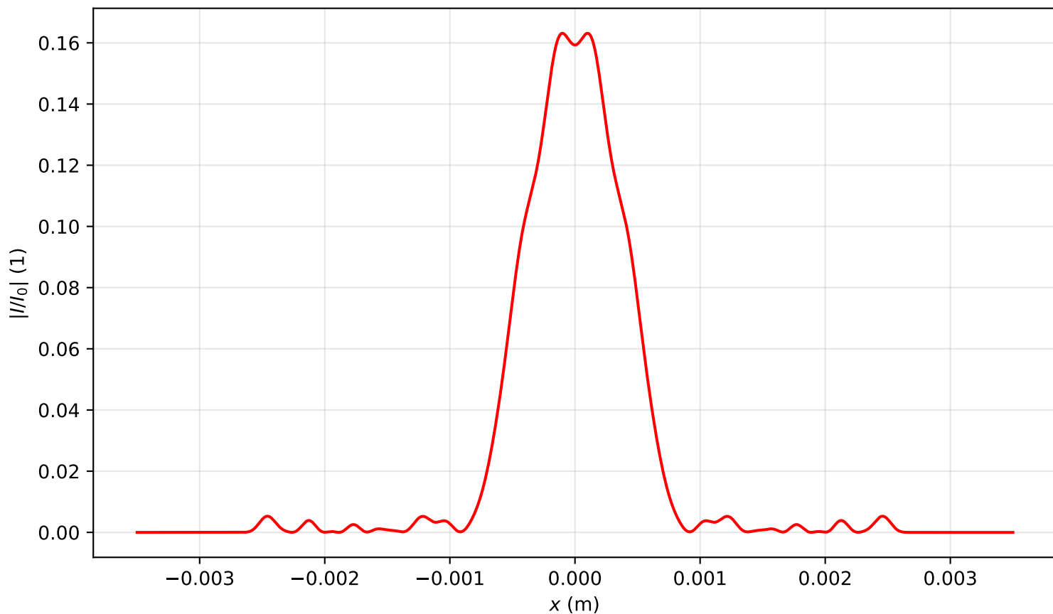
Intensity profile I(x, y = 0, z = 2.070)/I_0 , P_{in}=5.0P_{cr} , artificial time
